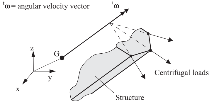
Figure 5.4-1: Convention used for centrifugal loading
