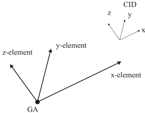
Figure 2.6-3: 6-DOF spring element with single node
