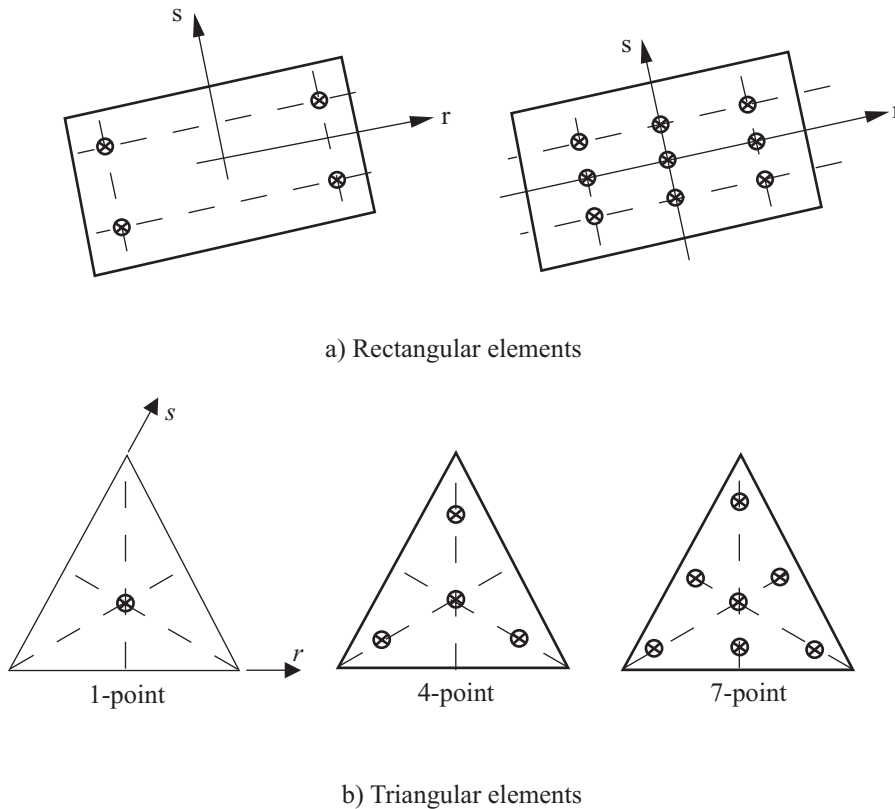
Figure 2.4-4: Integration point positions for 2-D solid elements
