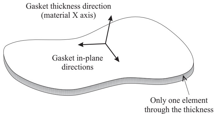
Figure 3.8-1: Schematic of gasket
