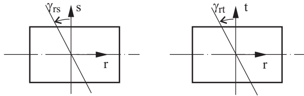
Figure 2.2-5: Assumptions of shear deformations through element thickness for nonlinear elasto-plastic beam element
