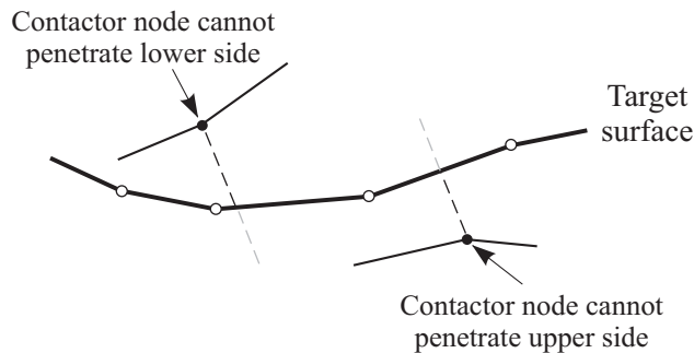
Figure 4.1-4: Double-sided contact
