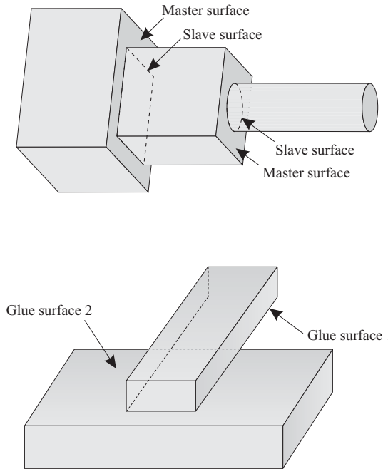
Figure 5.9-2: Examples of master and slave glue surfaces
