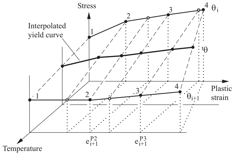
b) Yield curves
