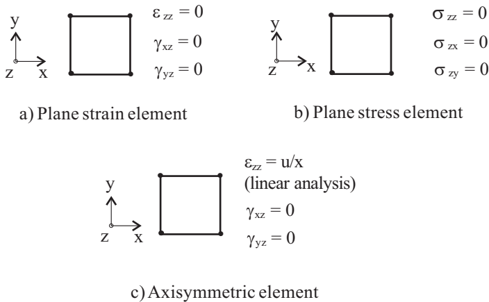
Figure 2.4-2: Basic assumptions in 2-D analysis (assuming element lies in X-Y plane)
