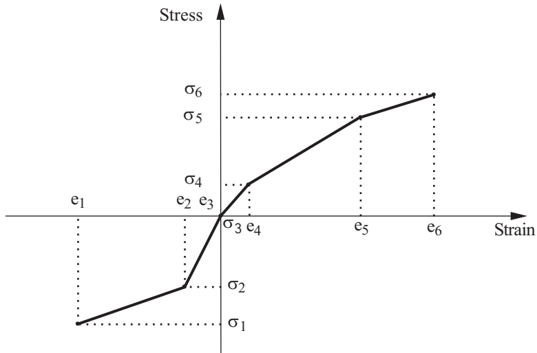
Figure 3.3-2: Nonlinear elastic material for rod elements
