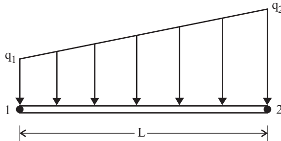
(a) Beam distributed loading
