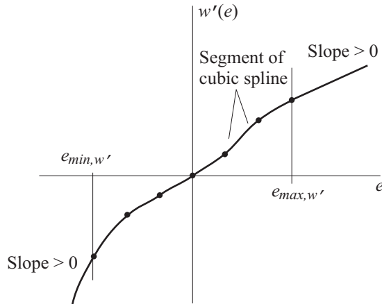
Figure 3.7-3: w'(e) spline
