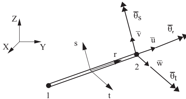
Figure 2.2-2: Conventions used for 2-node Hermitian beam element
