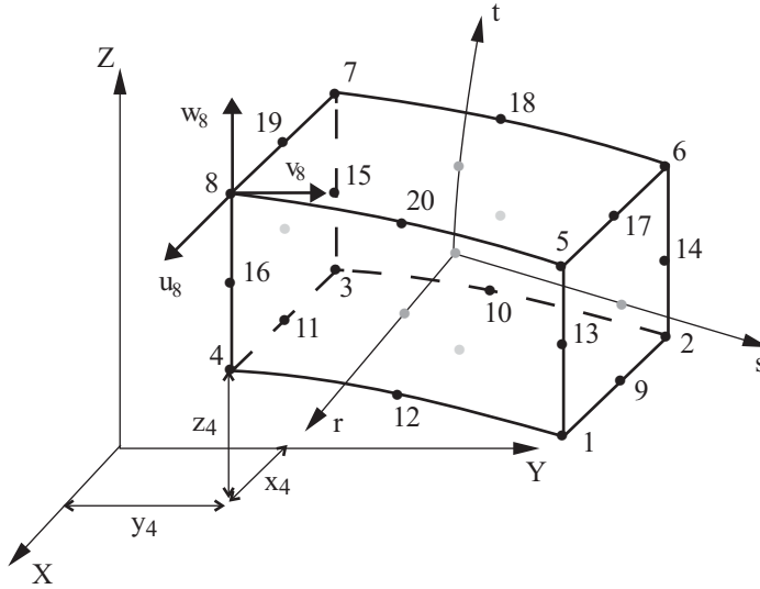
Figure 2.5-2: Conventions used for the nodal coordinates and displacements of the 3-D solid element
