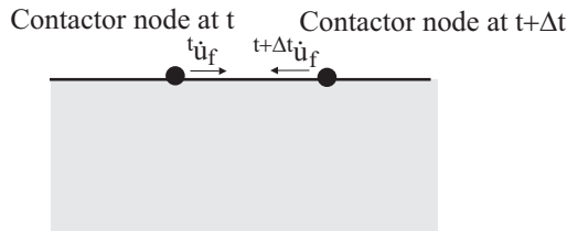
Figure 4.8-18: Reverse sliding due to too large time step in Solution 701
