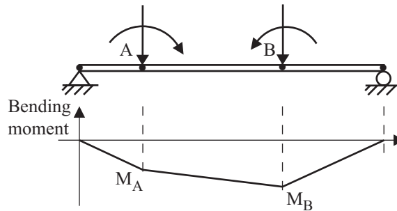
b) Finite element bending moment diagram using 3 beam elements
