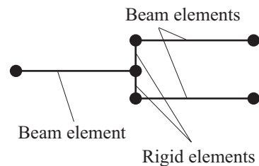
Figure 2.2-3: Use of rigid elements for modeling off-centered beams
