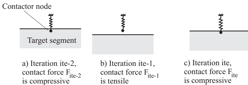
Figure 4.8-9: Iterations when tensile contact is used
