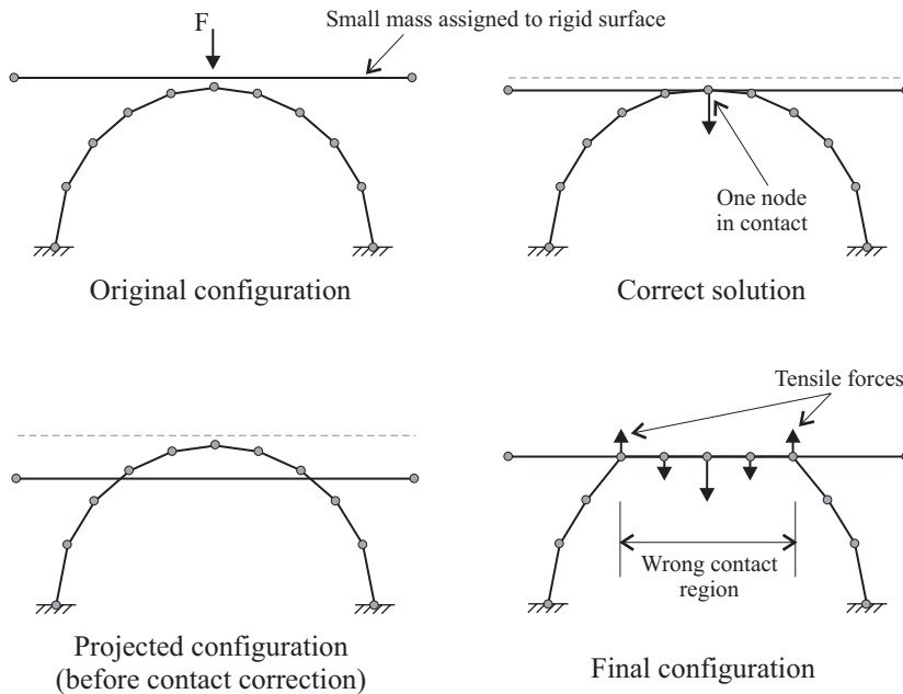
Figure 4.7-5: Performance of kinematic contact algorithm when contact surfaces have a large mass mismatch
