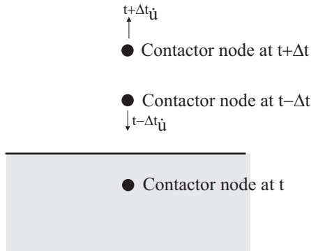
Figure 4.8-17: Contact reversal due to too large time step in Solution 701
