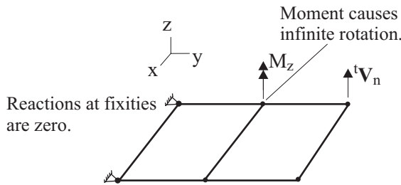
b) Moment applied in shell normal direction.
