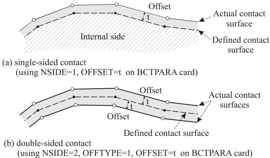
Figure 4.4-1: Contact surface offsets
