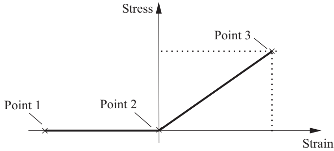
Figure 3.3-3: Nonlinear elastic material model corresponding to a tension-only cable
