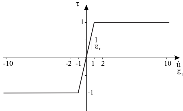
Figure 4.2-2: Frictional contact constraint function for new friction algorithm
