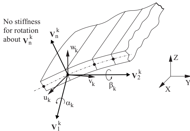
Figure 2.3-3: Shell degrees of freedom at node k
