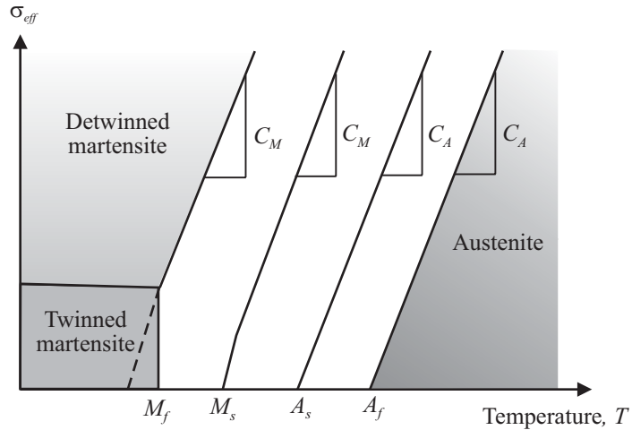
Figure 3.9-1: SMA stress-temperature phase diagram
