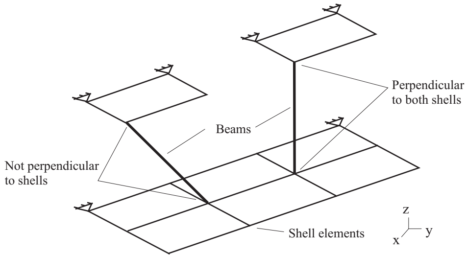
Figure 2.3-10: Beams intersecting shell elements
