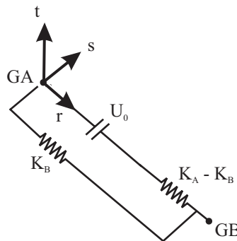
Figure 2.8-1: CGAP element coordinate system
