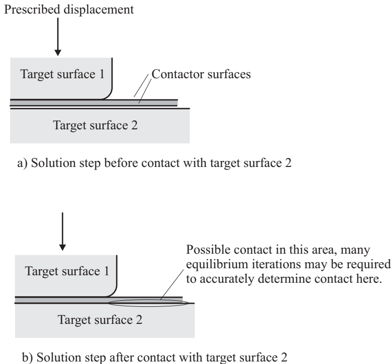
Figure 4.8-19: Establishment of contact over a large area during a solution step
