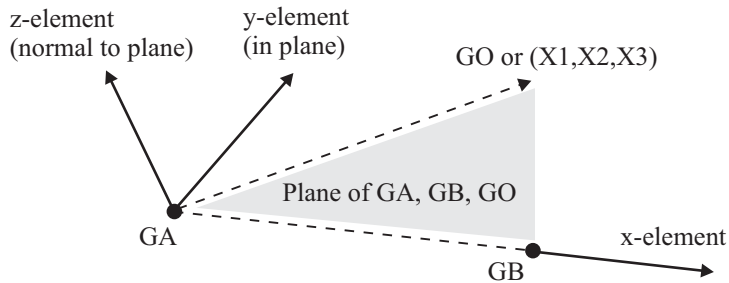
Figure 2.6-6: 6-DOF spring element with two non-coincident nodes
