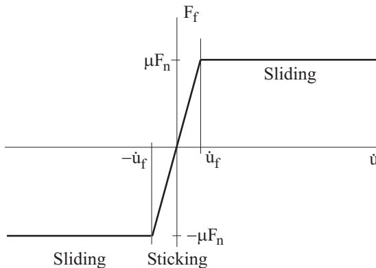
Figure 4.8-11: Friction force vs. velocity
