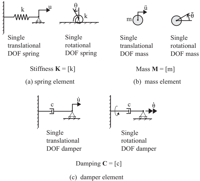
Figure 2.6-1: Single degree of freedom scalar elements
