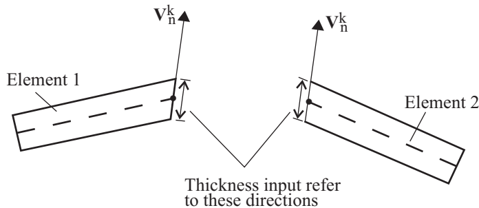
Figure 2.3-15: Program-calculated director vector at thermal shell nodes
