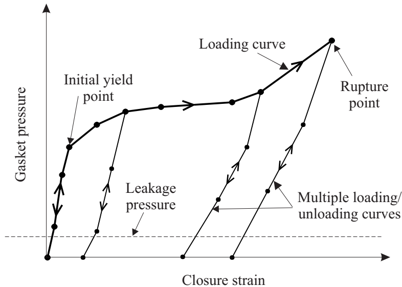
Figure 3.8-2: Pressure-closure relationship for a gasket material
