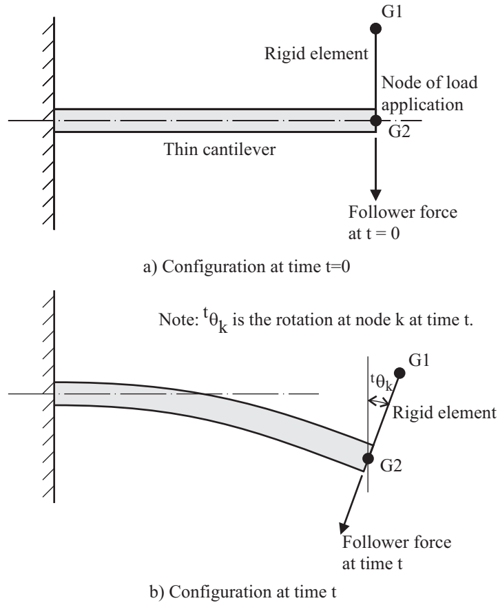
Figure 5.2-1: Example of the use of a rigid element to establish the follower load direction
