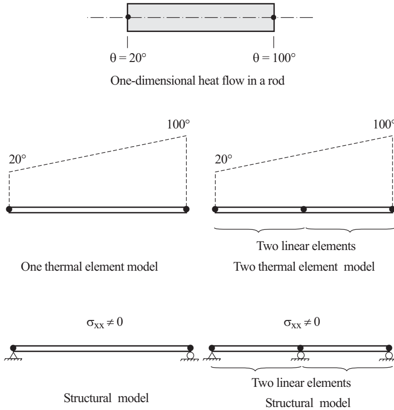
Figure 9.1-1: Simple problem to schematically demonstrate solution inaccuracies that can arise due to discretizations used in heat flow and stress analyses
