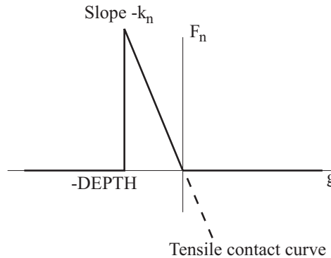
Figure 4.8-7: Normal contact force vs. gap
