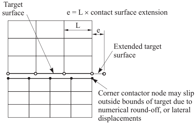
Figure 4.4-6: Contact requiring contact surface extension
