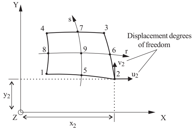
Figure 2.4-3: Conventions used for the 2-D solid element (assuming element lies in X-Y plane)
