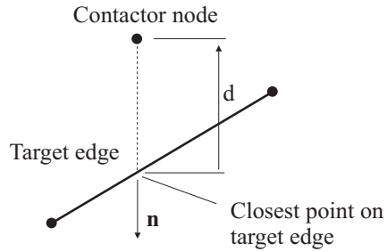
b) Interaction between contactor node and target edge
