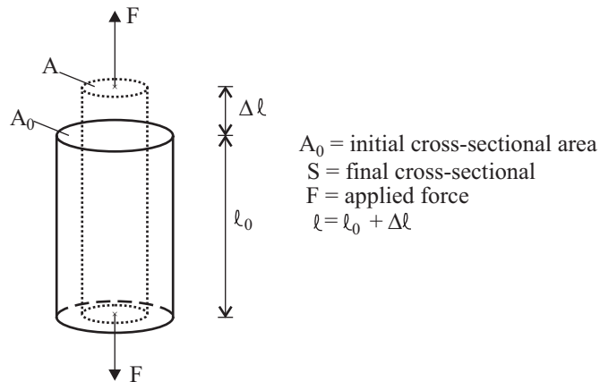
Figure 3.1-1: Rod under uniaxial tension
