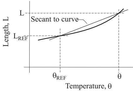
Figure 3.1-3: Length of bar vs. temperature
