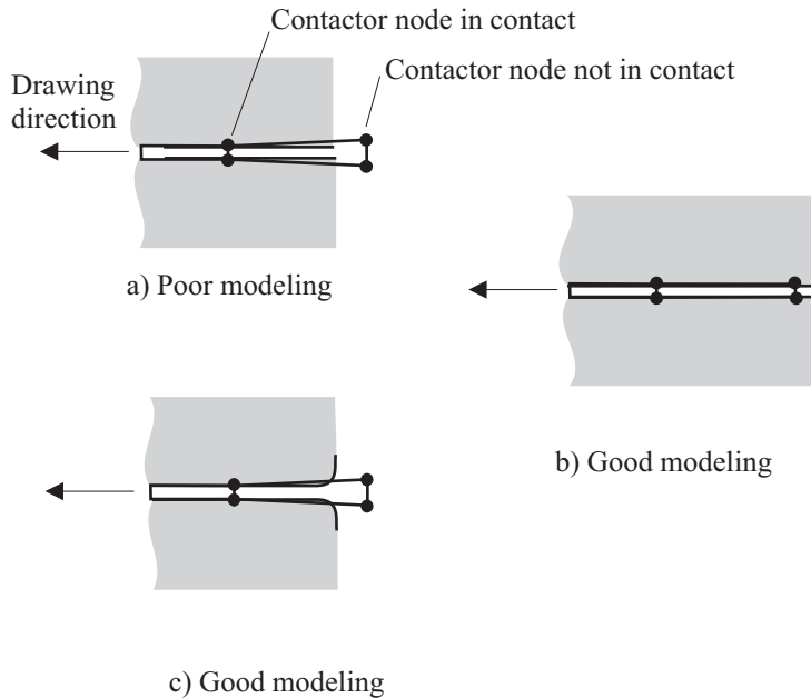
Figure 4.8-21) Contactor nodes suddenly coming into contact
