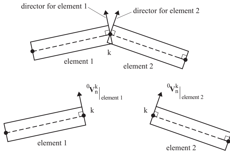
Figure 2.3-8: 6 degree of freedom shell node with separate director vectors at node k (each vector is used as a director vector for the respective element)
