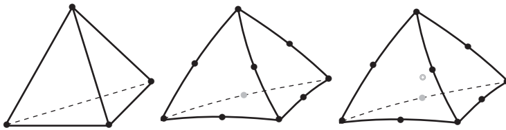
(b) 4-, 10- and 11-node tetrahedral elements (CTETRA)
