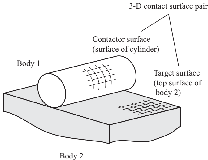
Figure 4.1-1: Typical contact surfaces and contact pair
