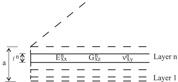
Figure 2.3-13: Multilayered shell
