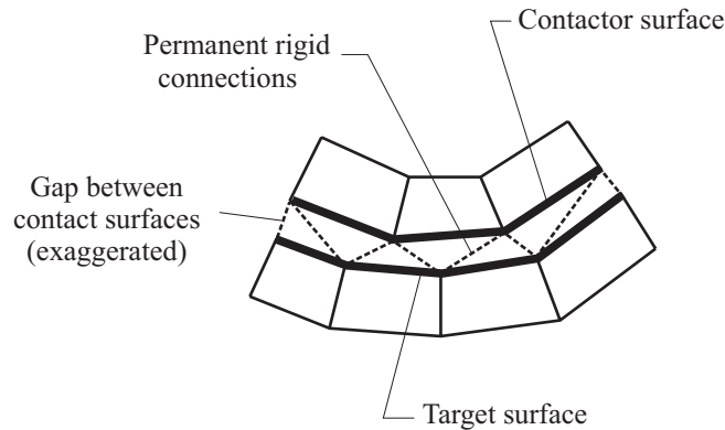
Figure 4.1-5: Tied contact option
