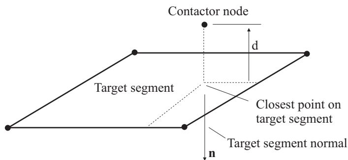
a) Interaction between contactor node and target segment
