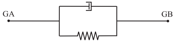
Figure 2.8-2: BUSH1D element
