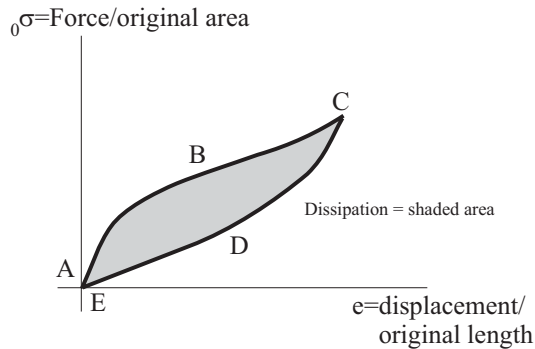
Figure 3.7-7: Dissipation in Mullins effect in a loading-unloading cycle
