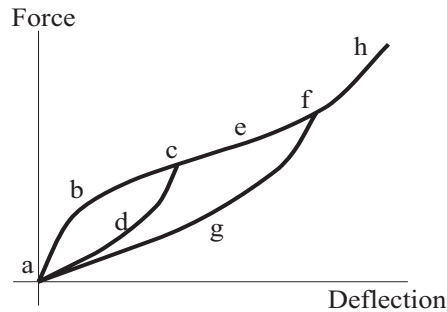
Figure 3.7-5: Mullins effect loading-unloading-reloading curves
