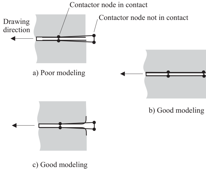
Figure 4.8-20: Contactor nodes suddenly coming into contact
