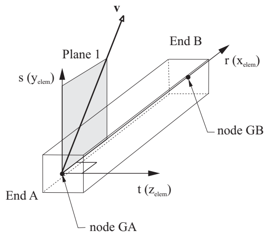
Figure 2.2-1: Beam element
