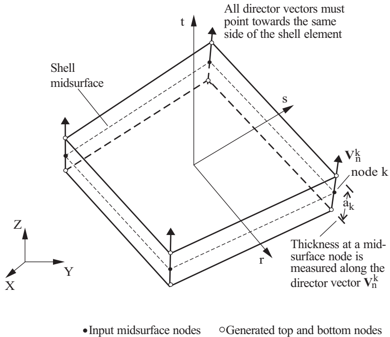
Figure 2.3-14: Description of the thermal shell element
