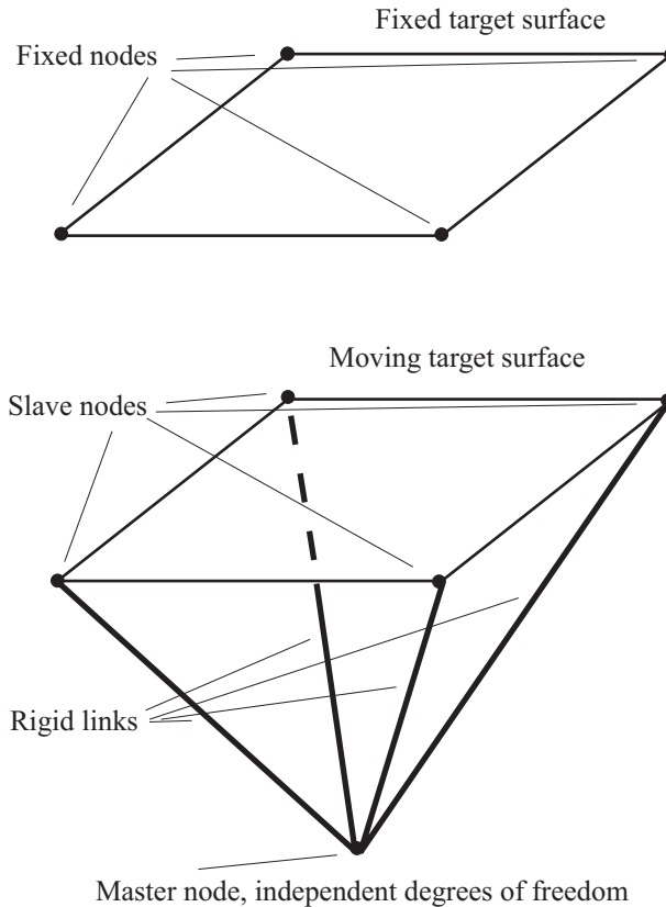
Figure 4.8-12: Modeling of fixed and moving target surfaces
