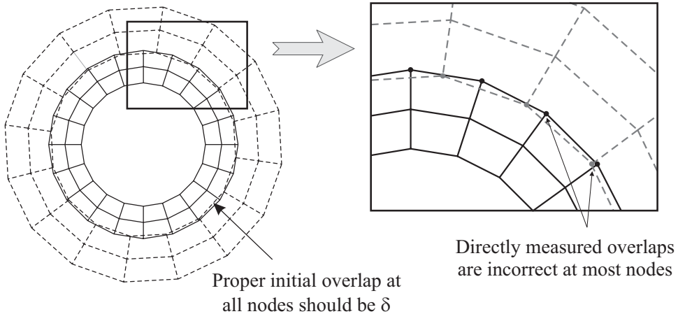
Figure 4.4-5: Significance of gap override for curved non-matched geometries
