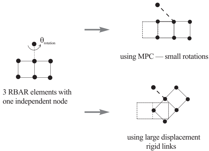
Figure 2.7-1: Difference between small displacement MPC and large displacement rigid links
