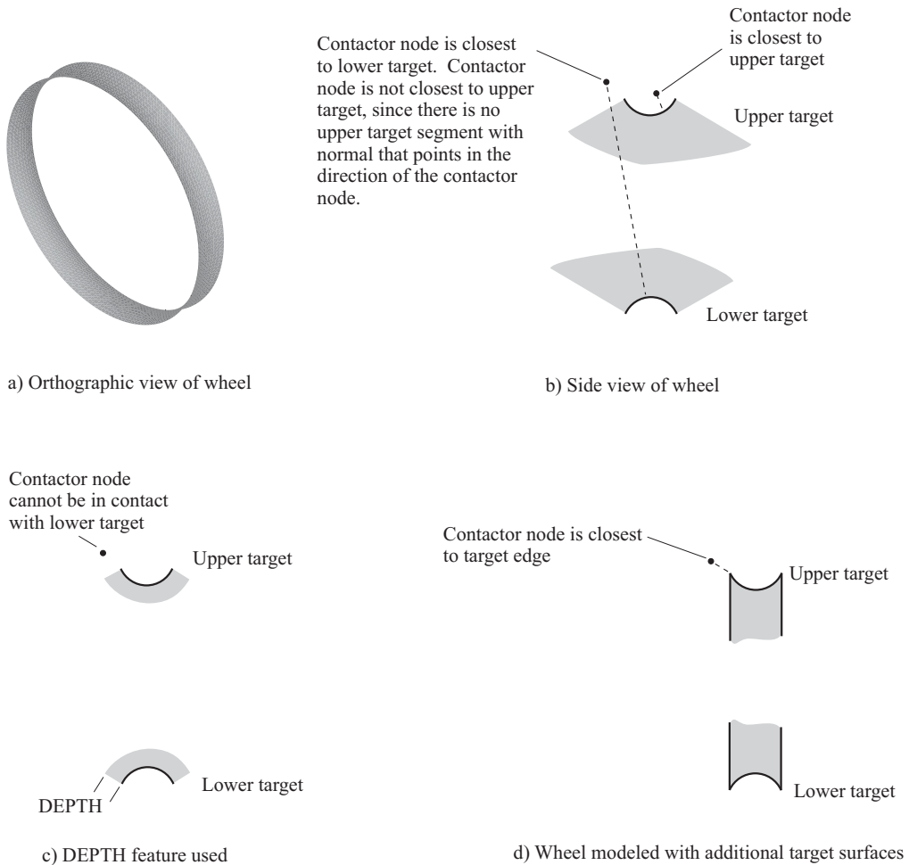
Figure 4.8-13: Modeling of a wheel
