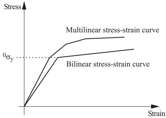
Figure 3.4-1: von Mises model
