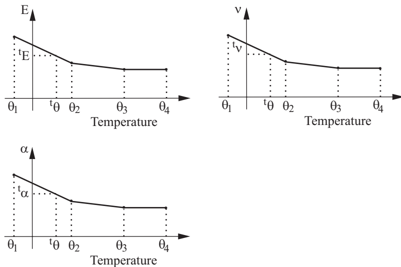
Figure 3.5-1: Variation of material properties for thermo-elastic model
