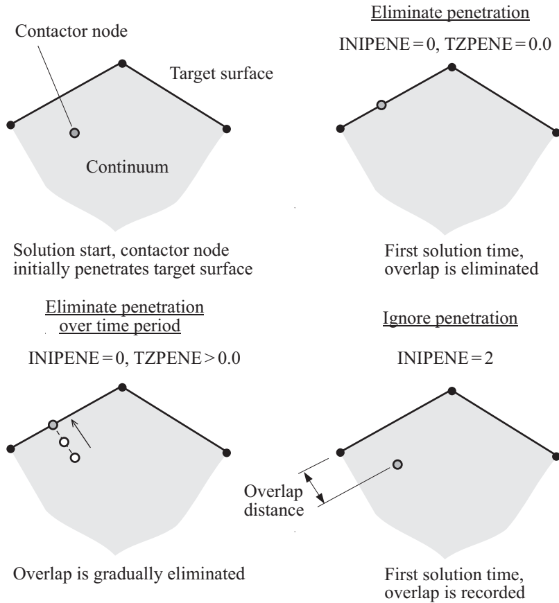
Figure 4.4-4: Initial penetration options
