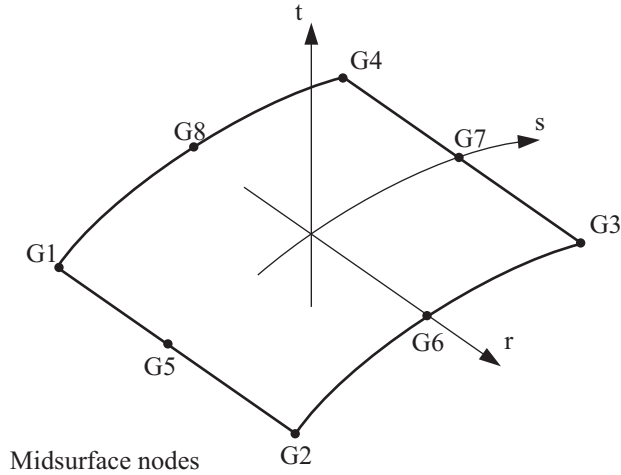
Figure 2.3-2: Some conventions for the shell element; local node numbering; local element coordinate system
