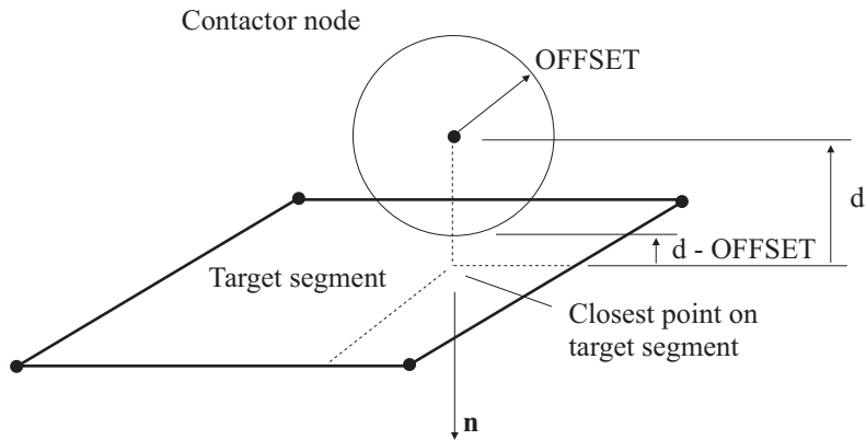
Figure 4.8-6: Interaction between contactor node and target segment, spherical offsets
