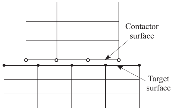
Figure 4.7-2: Target selection for surfaces of different sizes
