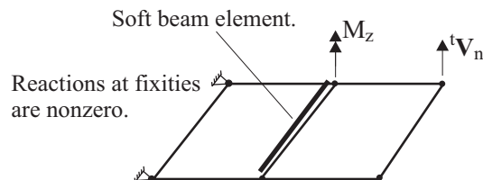
Figure 2.3-11: Soft beam element takes applied moment
