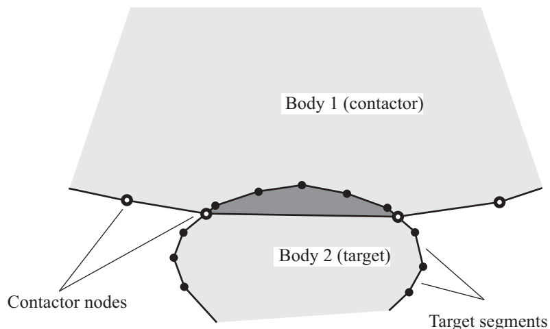
Figure 4.7-1: Effect of incorrect contactor-target selection due to mesh density
