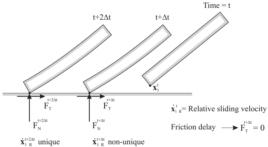
Figure 4.4-8: Friction delay feature
