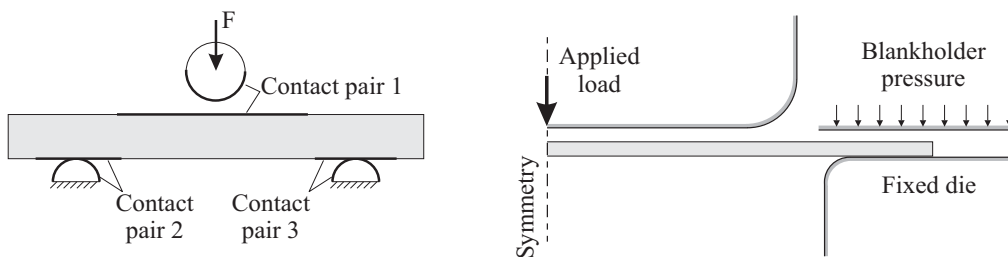
Figure 4.7-7: Examples of improperly supported bodies
