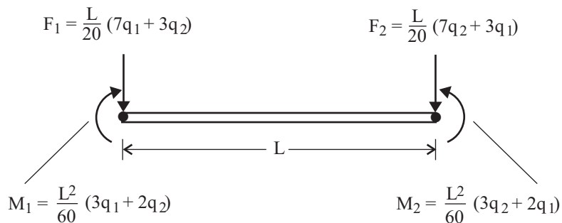
(b) Fixed-end forces/moments representation
