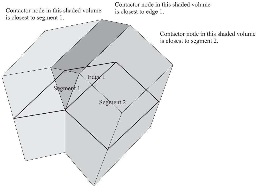
Figure 4.8-5: Interaction of contactor node with target segments and edges
