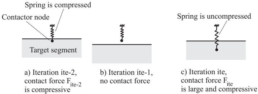
Figure 4.8-8: Iterations when tensile contact is not used
