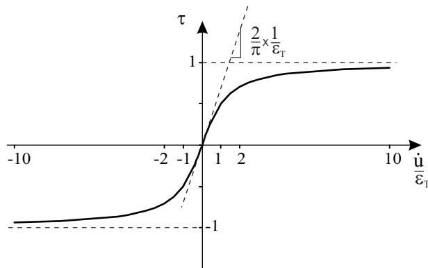
Figure 4.2-3: Frictional contact constraint function for old friction algorithm
