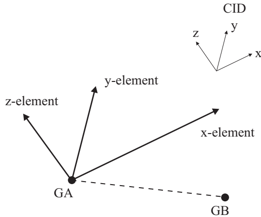
Figure 2.6-5: 6-DOF spring element with two non-coincident nodes
