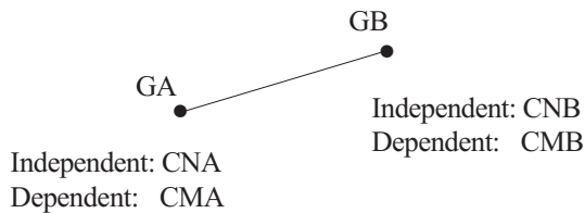
Figure 2.7-2: Relevant parameters in the RBAR rigid element
