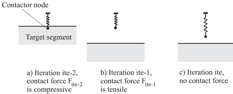
Figure 4.8-10: Iterations when tensile contact is used, converged solution not in contact
