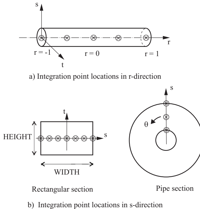
Figure 2.2-6: Integration point locations in elasto-plastic beam analysis
