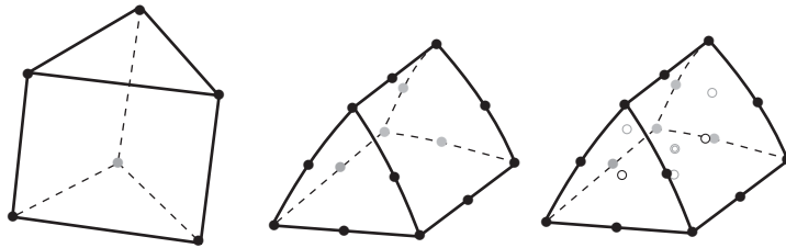
(c) 6-, 15-, and 21-node wedge elements (CPENTA)
