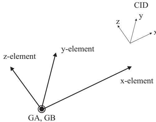
Figure 2.6-4: 6-DOF spring element with two coincident nodes
