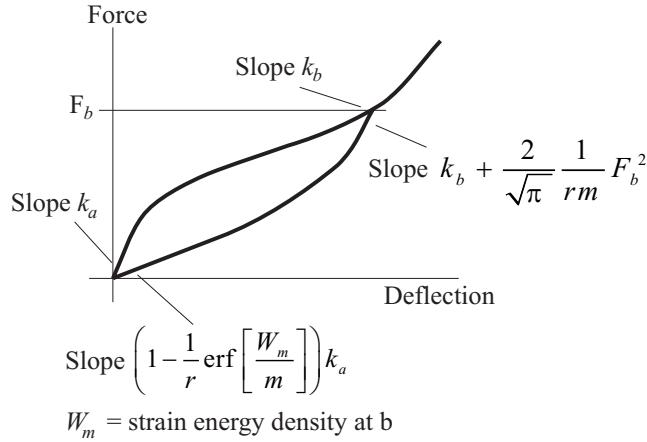
Figure 3.7-6: Dependence of reloading curve on Mullins effect material constants It can also be shown that the dissipation of a loading-unloading cycle, as shown in Fig 3.7-7, can be written as
