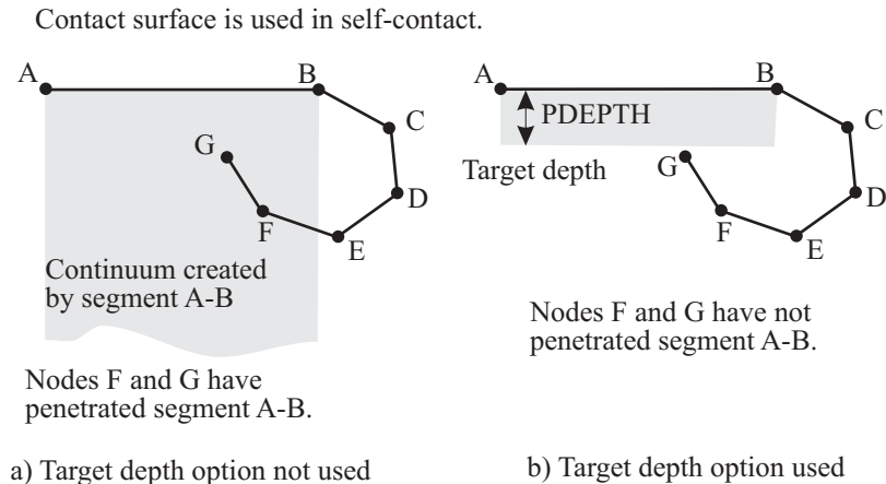
Figure 4.4-3: Contact surface depth.
