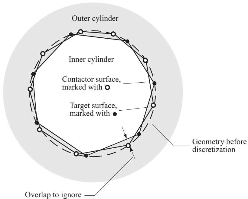
Figure 4.7-3: Analysis of contact between concentric cylinders, initial penetration is ignored
