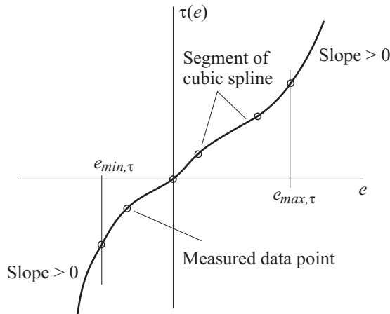
Figure 3.7-2: Uniaxial tension/compression stress-strain spline
