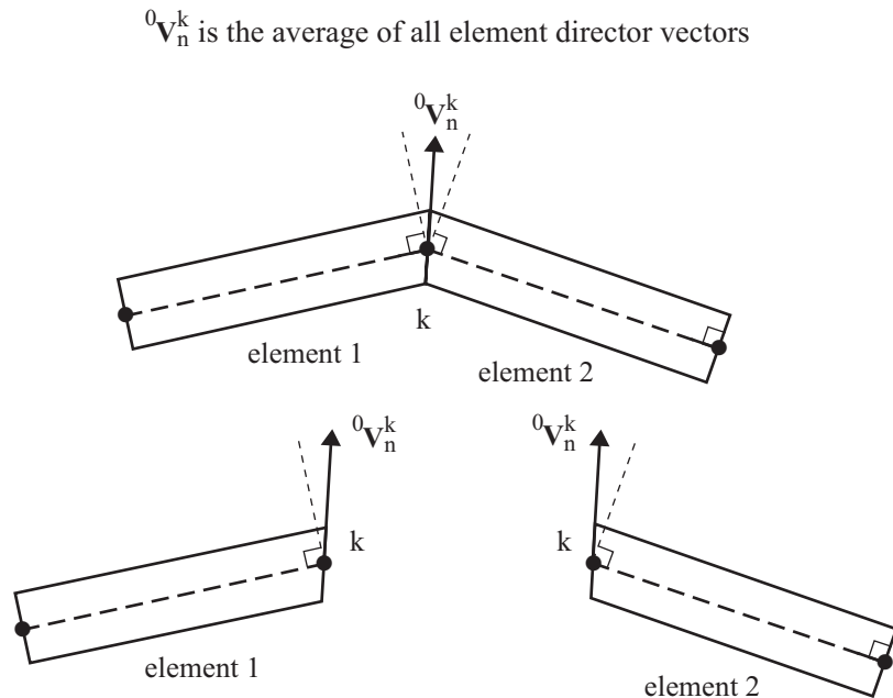
Figure 2.3-7: 5 degree of freedom shell node with unique vector at node k
