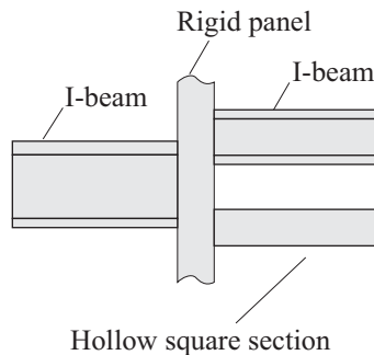
Figure 2.2-3: Use of rigid elements for modeling off-centered beams
