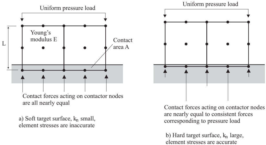
Figure 4.8-16: Higher-order elements and rigid-target contact
