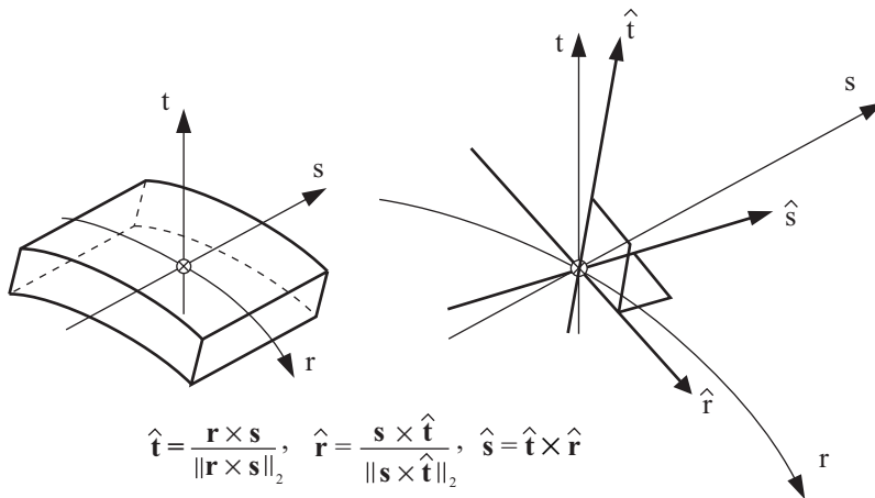
b) Definition of the midsurface Cartesian system (\hat{\mathbf{r}}, \hat{\mathbf{s}}, \hat{\mathbf{t}}) at an integration point
