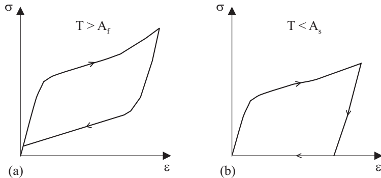
Figure 3.9-3: Schematic of stress-strain curves for shape-memory alloys (a) superelasticity; and (b) shape memory effect
