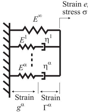
Figure 3.7-4: Equivalent 1D model for viscoelastic effects
