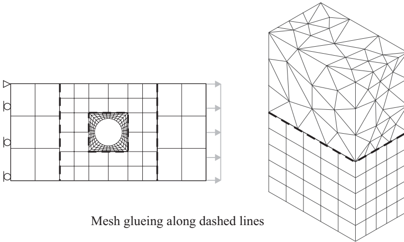
Figure 5.9-1: Examples requiring mesh gluing
