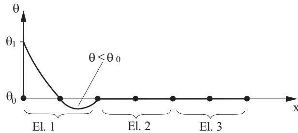
Figure 5.6-1: Interpolation of temperature boundary conditions
