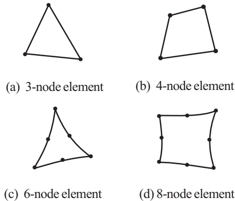
Figure 2.3-1: Shell elements in Advanced Nonlinear Solution
