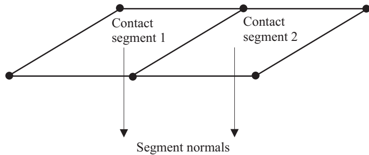
a) Contactor segments without offsets. Segment normals are not used.
