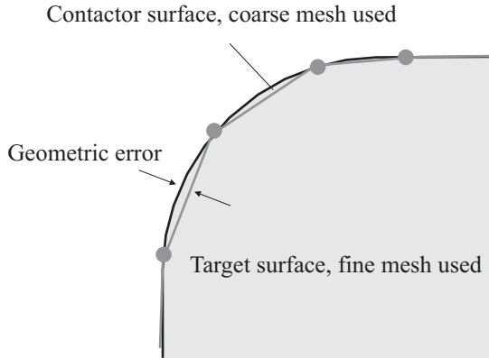
Figure 4.8-15: Modeling of a curved target surface
