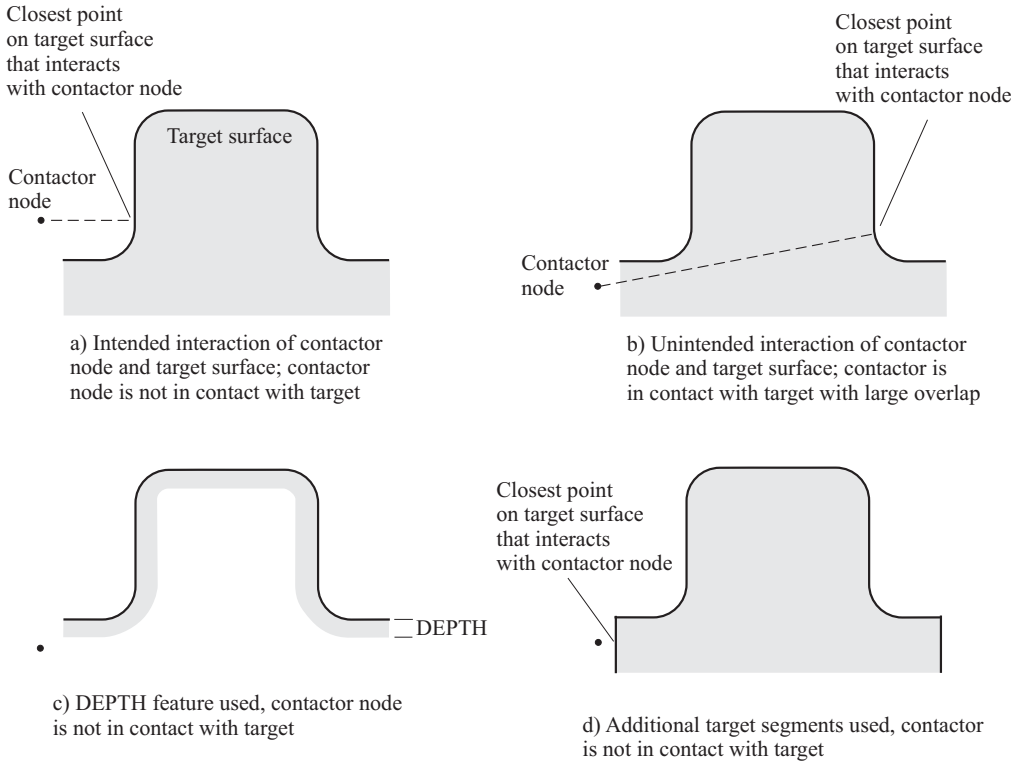
Figure 4.8-14: Modeling of a punch
