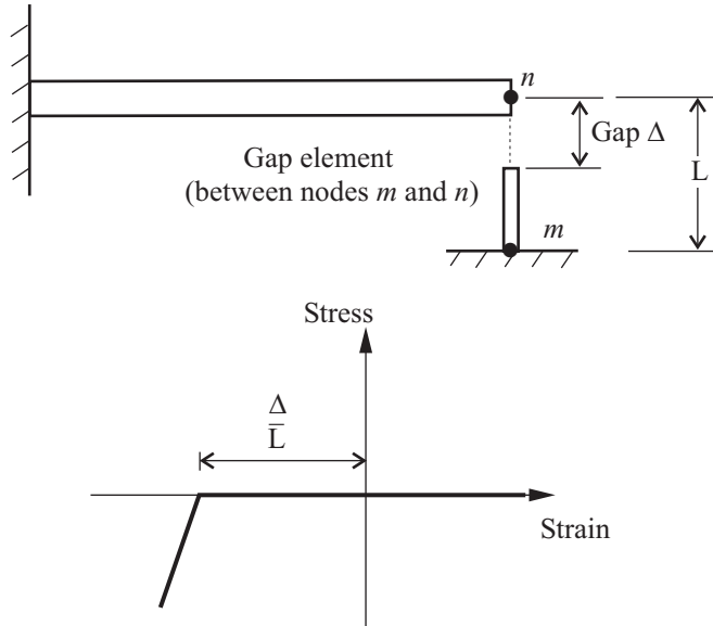
Figure 3.3-4: Modeling of gaps
