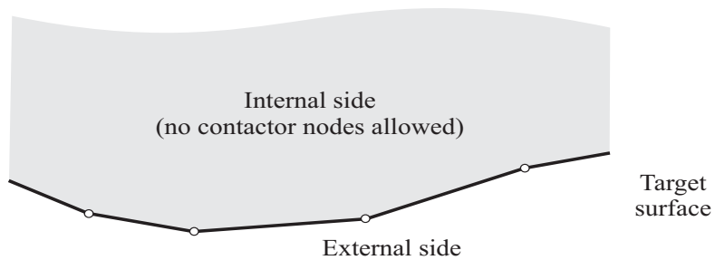
Figure 4.1-3: Single-sided contact surface
