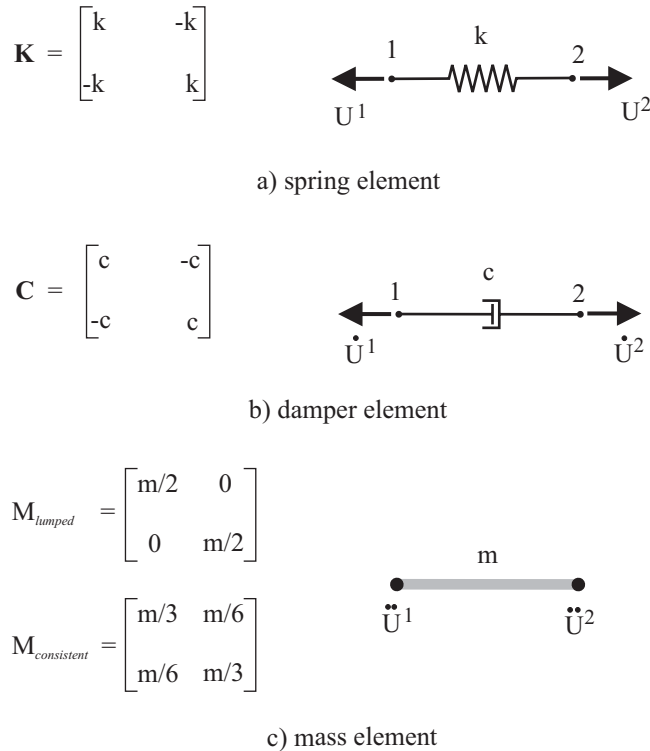
Figure 2.6-2: Two-degrees-of-freedom scalar elements
