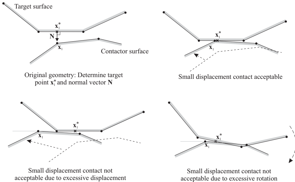
Figure 4.1-6: Small displacement contact feature
