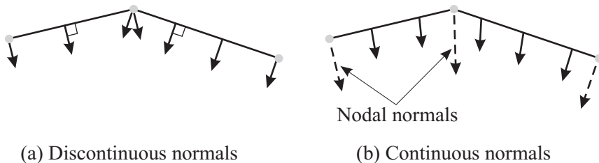
Figure 4.4-2: Contact surface normals
