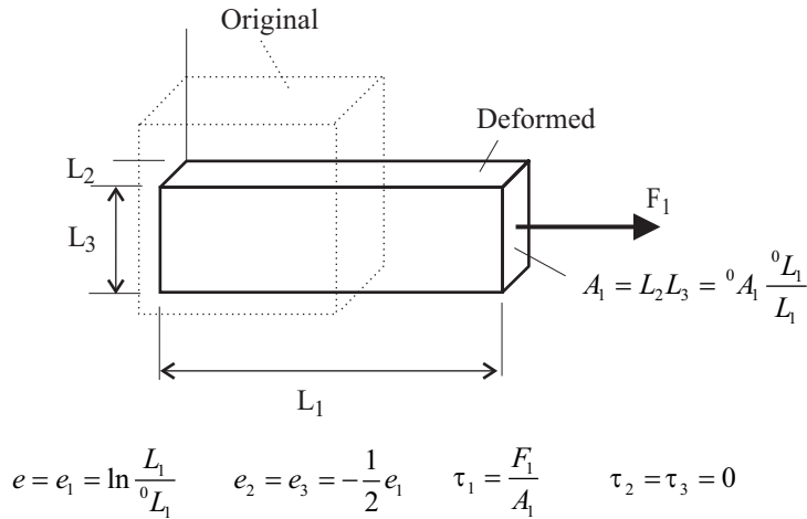
Figure 3.7-1: Uniaxial tension/compression test
