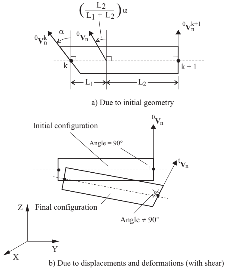
Figure 2.3-4: Examples of director vectors not normal to the shell midsurface
