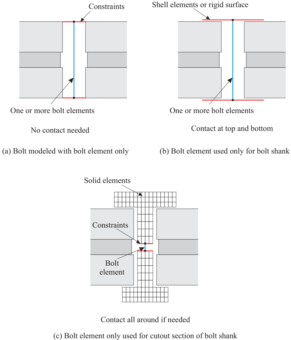
Figure 10.7-2: Different bolt modeling techniques
