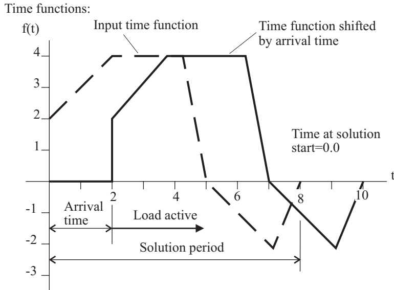
Figure 5.1-3: Example of the use of the arrival time option
