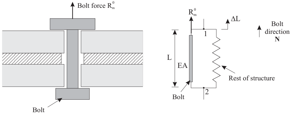
Figure 10.7-1: Schematic illustrating the bolt modeling feature
