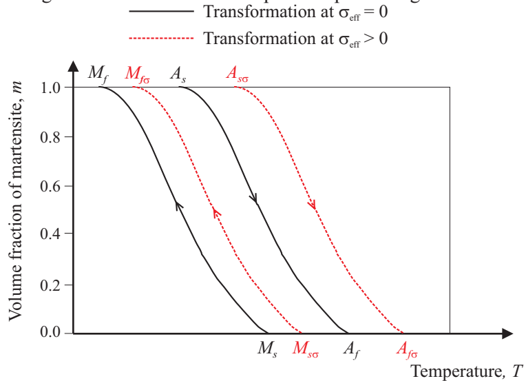
Figure 3.9-2: Volume fraction of martensite vs. temperature
