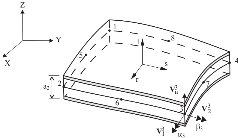
Figure 2.3-12: 8-node composite shell element
